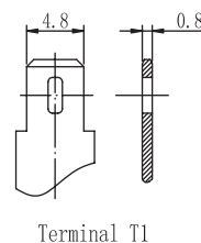
Terminal T1
